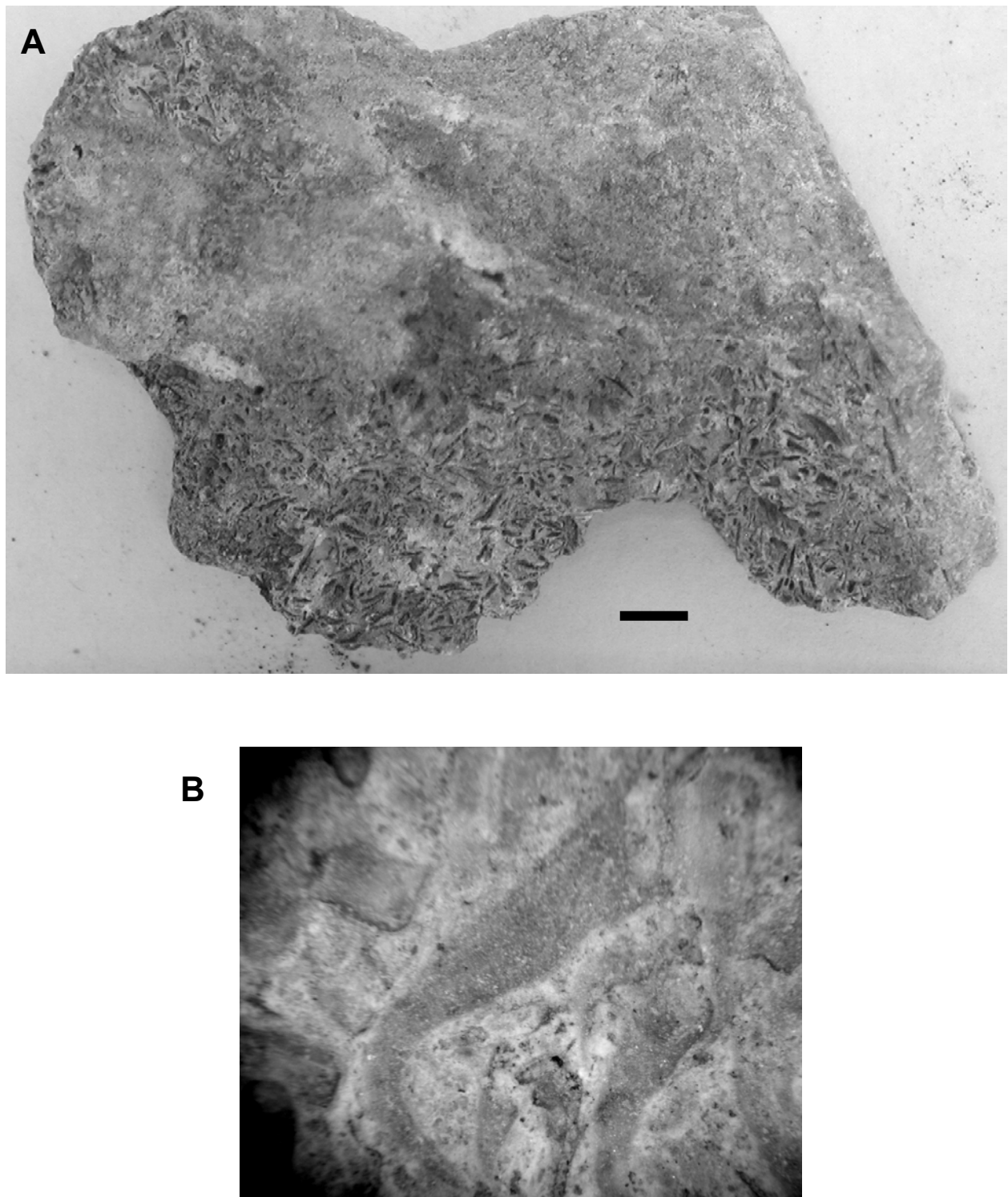
FIGURE 8. A. Dense amounts of coleoid cephalopod tentacle hooklets, interpreted as gastric contents of the pliosaur, were found within the matrix. The hooklets were preserved with the original chitin intact in the sandy matrix. Scale bar equals 5 mm. B. Hooklets also preserved as calcite-filled molds in the matrix. Field of view approximately 5 mm wide.
